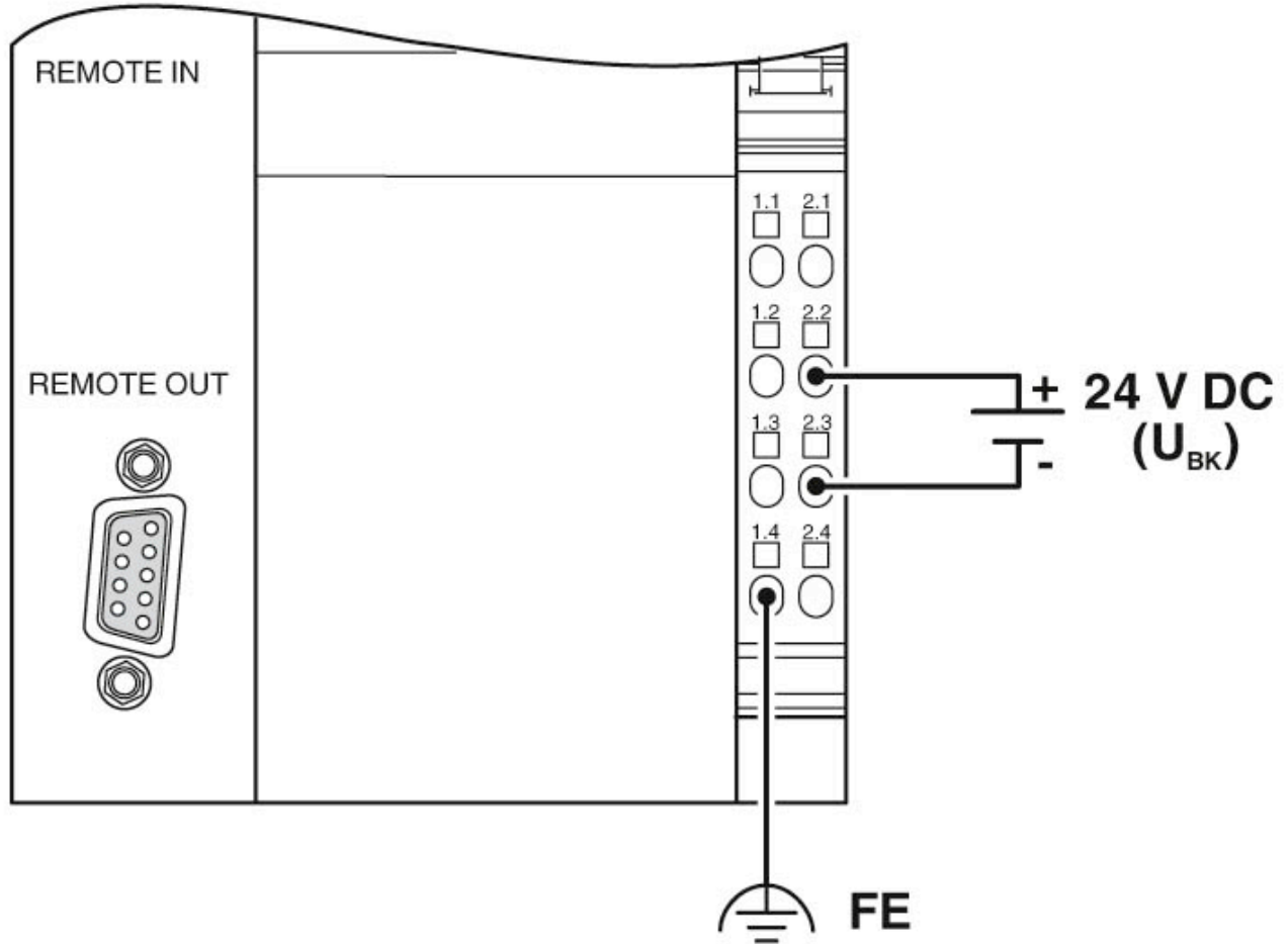
Connection diagram
